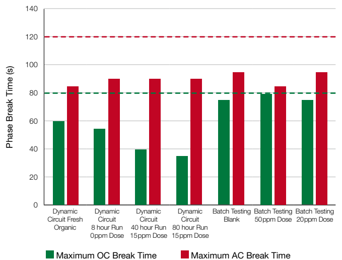
Fig. 2a Extraction and Strip Kinetics compatibility data and Fig. 2b Phase Break compatibility data for batch and dynamic circuit testing
